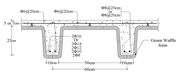
■ Cross Section of Green Waffle Slab Scale=1/10 Beam width=10 cm
