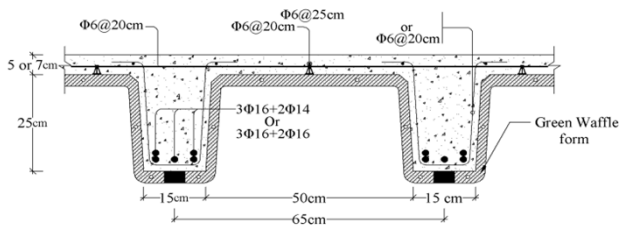
■ Cross Section of Green Waffle Slab Scale=1/10 Beam width=15 cm
