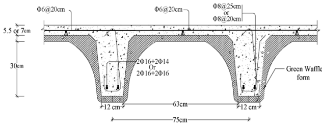
■ Cross Section of Green Waffle Slab Scale=1/10 Beam width=12 cm
