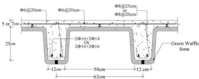
■ Cross Section of Green Waffle Slab Scale=1/10 Beam width=12 cm
